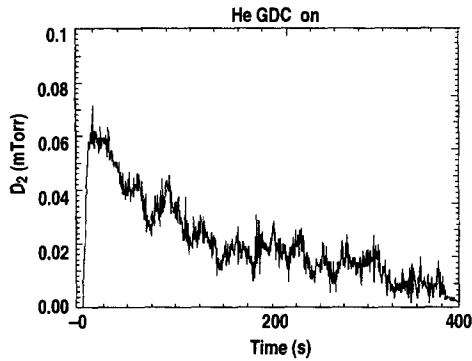
Fig. 3. Decay of deuterium partial pressure in ASDEX Upgrade during HeGDC after one of the first discharges of a run day (preceding discharge #6279).
